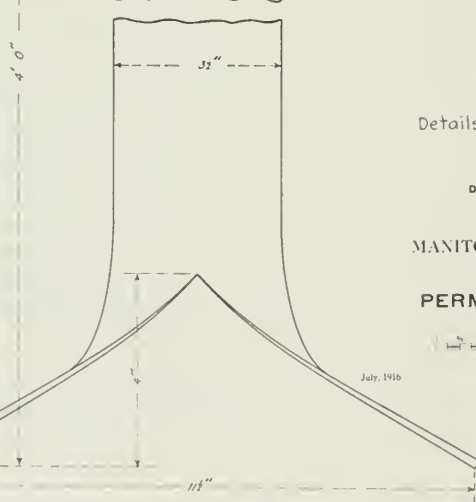
Details of Earth Bench Mark.
