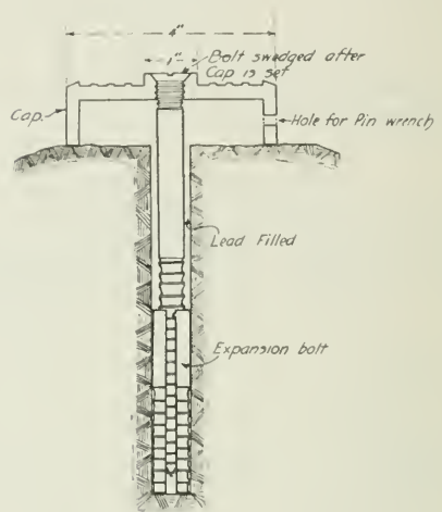
Details of Rock Bench Mark.
